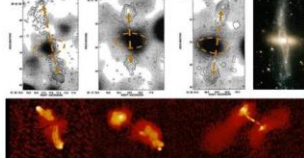
Figure 24, star formation and dying according to Quantum-FFF Theory.
