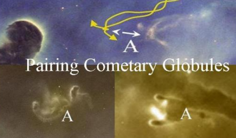
Figure 12, great misconceptions in astronomy and the solution with alternative electric dark matter black holes able to combine into Herbig haro objects with star ( or failed star) formation in between.
