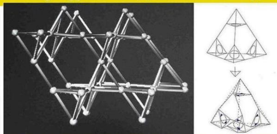
Simplified tetrahedral vacuum lattice structure (left), constructed by complex chiral tetrahedral building blocks (right). Each universe has to choose between a left- or righthanded rotation of its tetrahedral building blocks. Each chiral lattice has the Planck length and is supposed to be equipped with at least two oscillating massless new Higgs particles.
