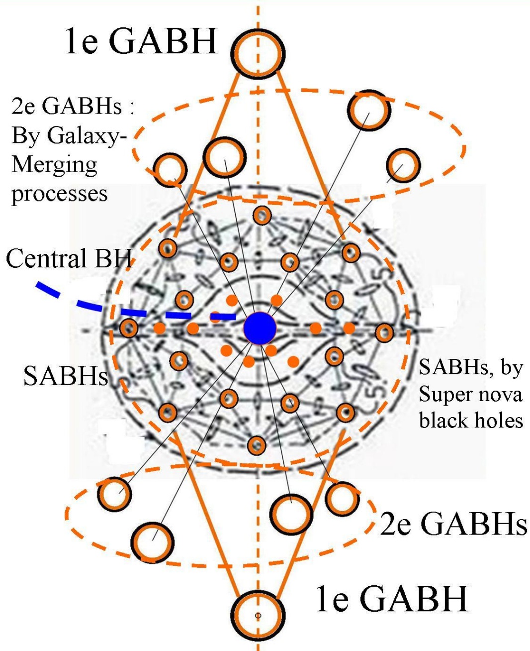
Figure: 30. Black hole families. 1e and 2e GABHs assumed to be the big bang nuclear explosion splinters. SABHs of different scales are assumed to be the results of primary and secondary etcetera, stellar Super Nova black holes. The central BH is assumed to be the beginning of one of the big crunch black holes.
